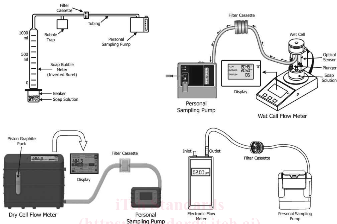
FIG. 1 Calibration Setup—Setting and Verifying Flow Rate for Personal Sampling Pump with Filter Cassette Using a Manual Bubble Burette (Top Left), Wet Cell Electronic Flow Meter (Top Right), Piston Dry Cell Flow Meter (Bottom Left), and Mass Flow Electronic Flow Meter (Bottom Right)
