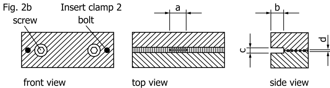
FIG. 2 Alternative Clamp for Constraining Rotation of the Geogrid Junction per 6.4
