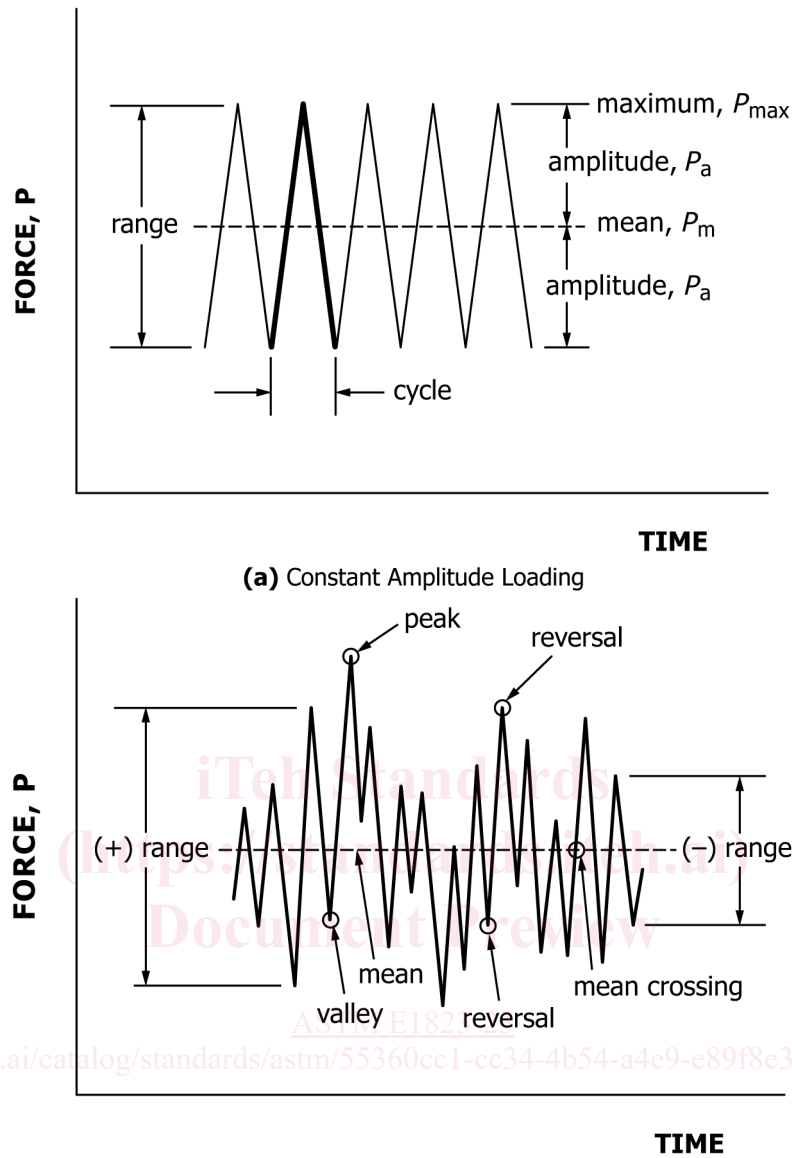
FIG. 4 Fatigue Loading Basic Terms
