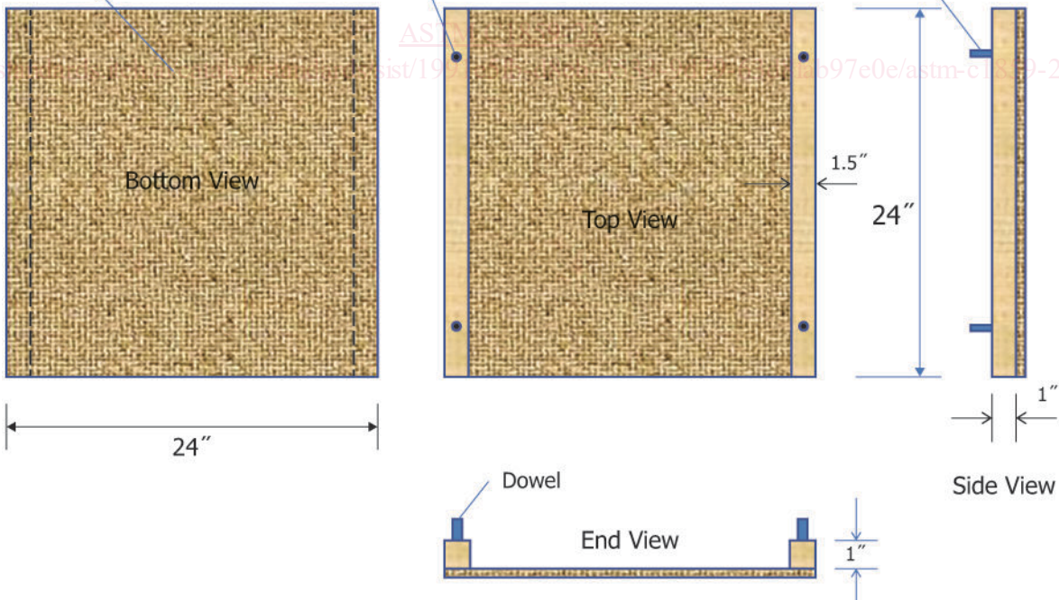
FIG. 2 Recommended Top and Bottom Test Frame (an Example)
