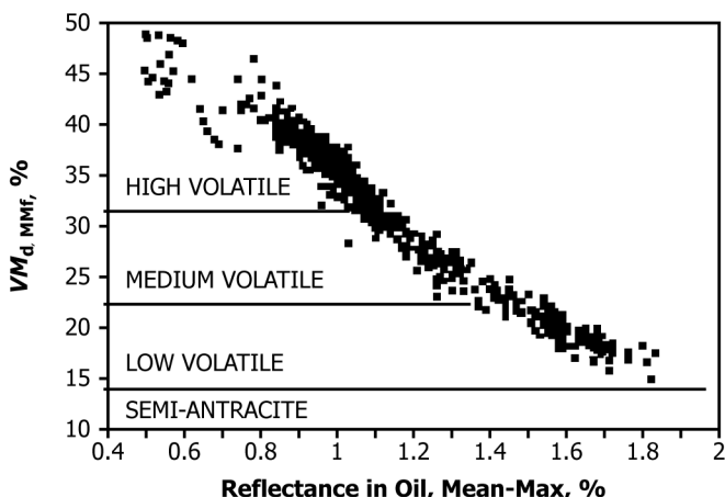
FIG. X1.1 Relation Between Rank of U.S. Coals and Vitrinite Reflectance
