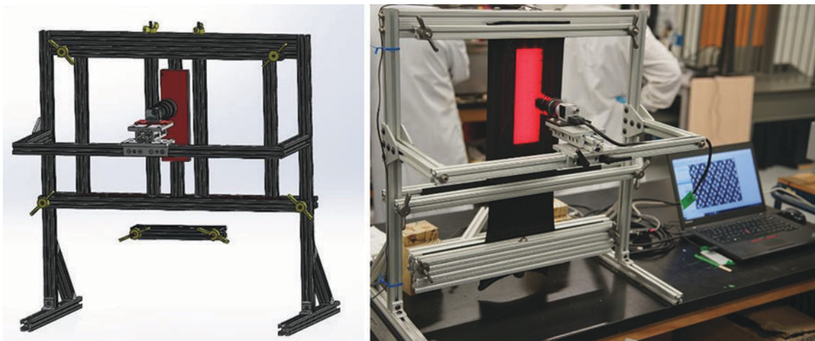
FIG. 2 Stretching Structure
