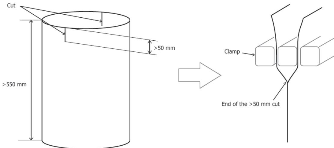
FIG. 4 Positioning of the Specimen in the Clamps
