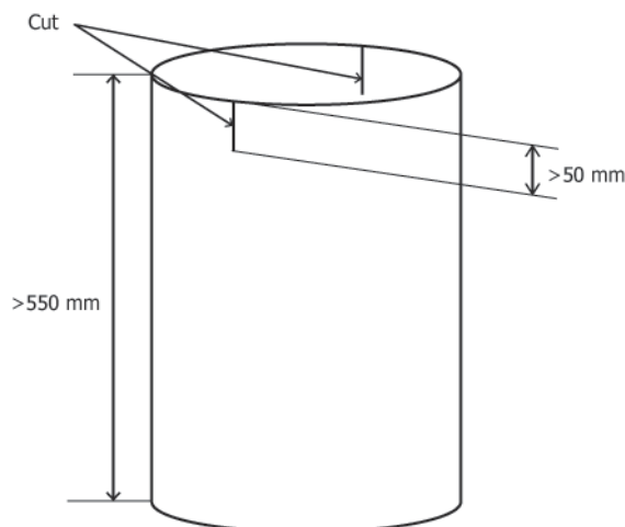
FIG. 3 Position of the Cuts
