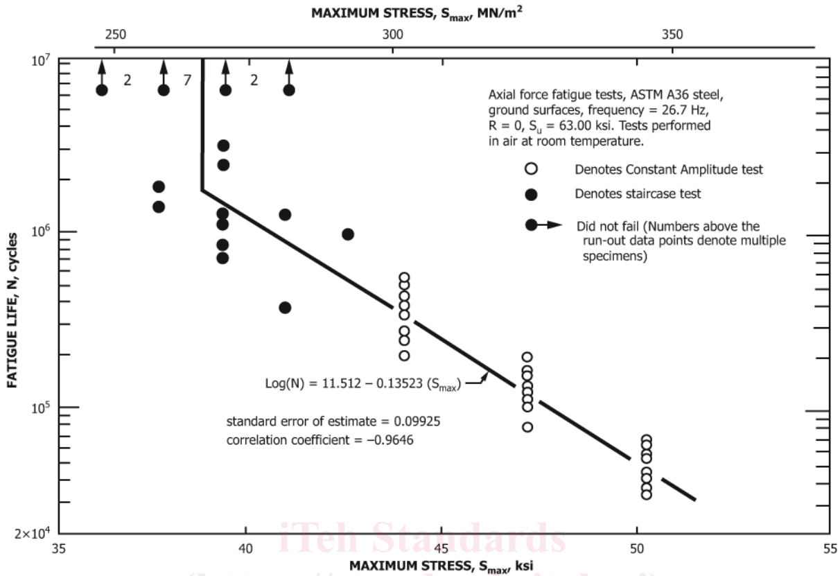
FIG. 2 S-N Diagram (alternative)
