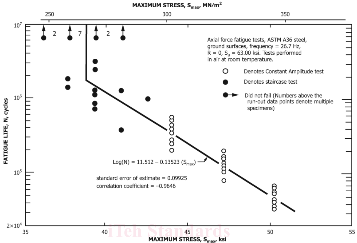
FIG. 2 S-N Diagram (alternative)
