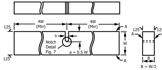
FIG. 4 Beam Specimen
