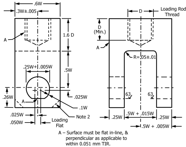
FIG. 2 Tension Test Clevis Design
