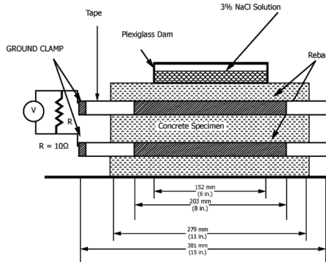
FIG. 2 Concrete Beam (Side View)
