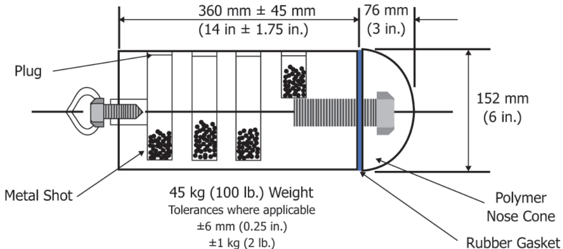
FIG. 1 Impactor Details
