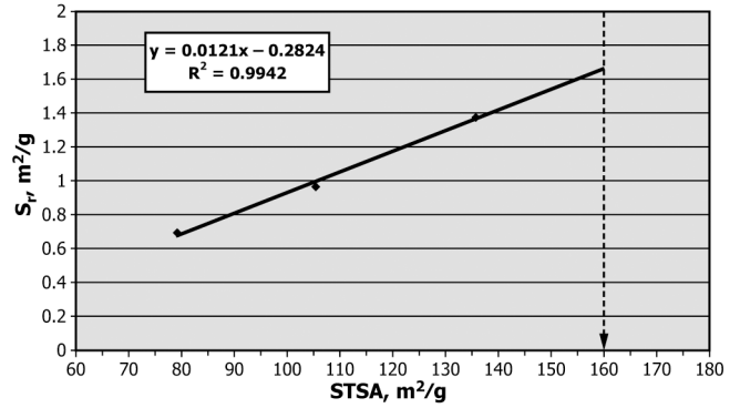
FIG. A1.2 Estimation of STSA S_r for Tread Product Using SRB-6
