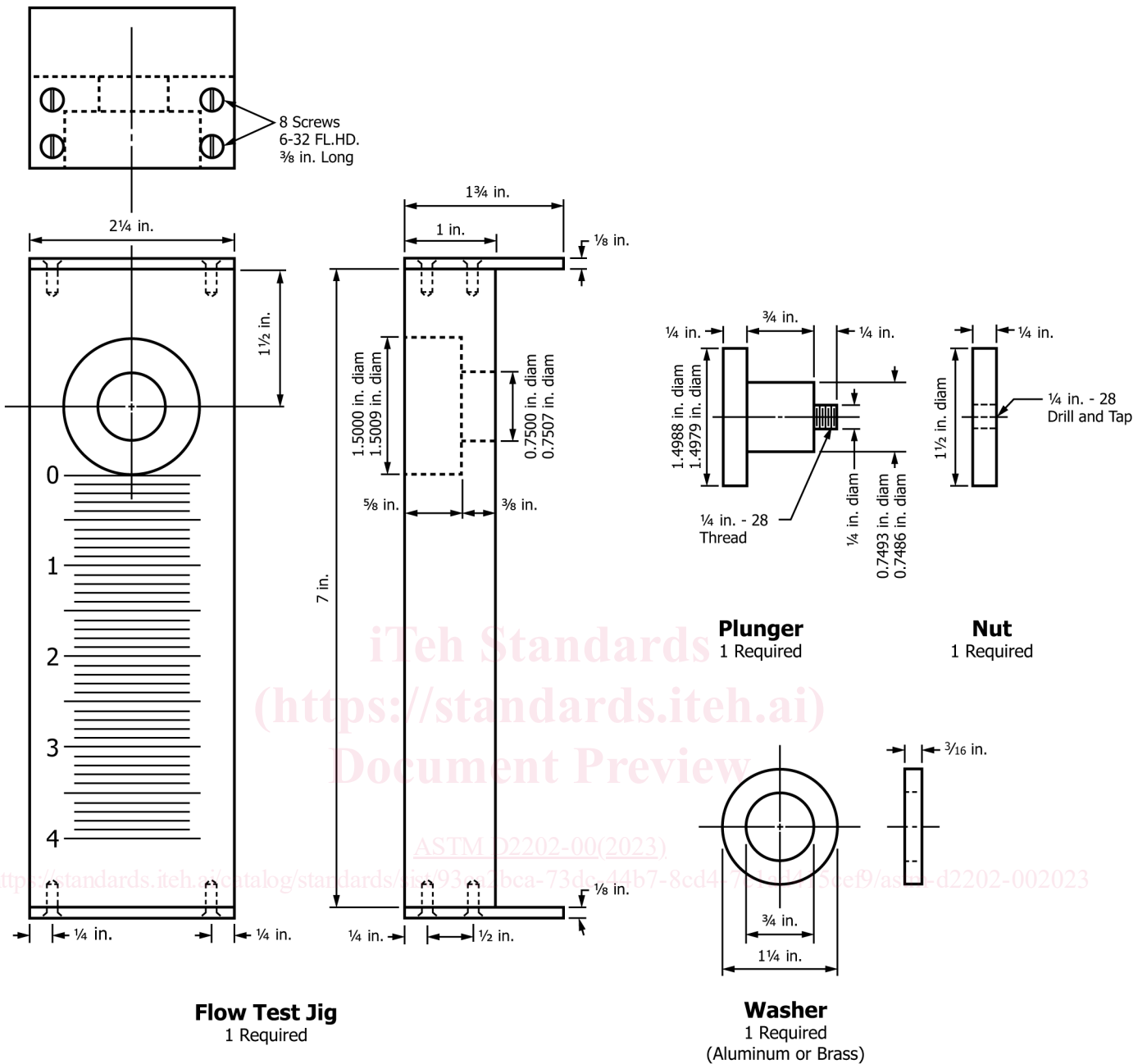
FIG. 2 Flow Test Jig (Inch-Pound Units)
