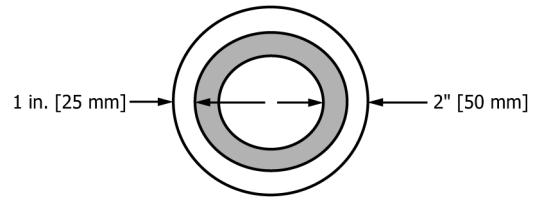
FIG. 1 Top View of Mortar Test Specimen
