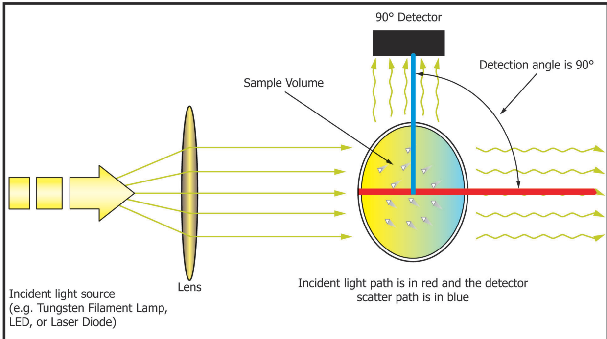
FIG. 1 The Photoelectric Nephelometer
