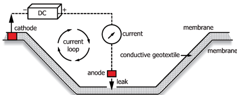
FIG. 1 Schematic of Leak Detection with Conducting Conductive Geotextile
