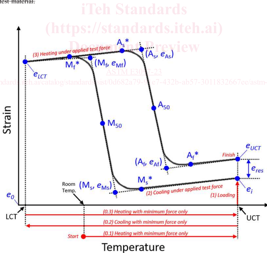
FIG. 1 Typical Constant Force Thermal Cycle and Test Methods Terms
