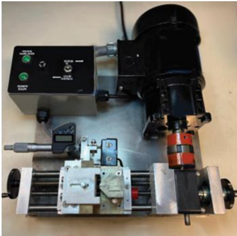
FIG. 2 Notching Machine
