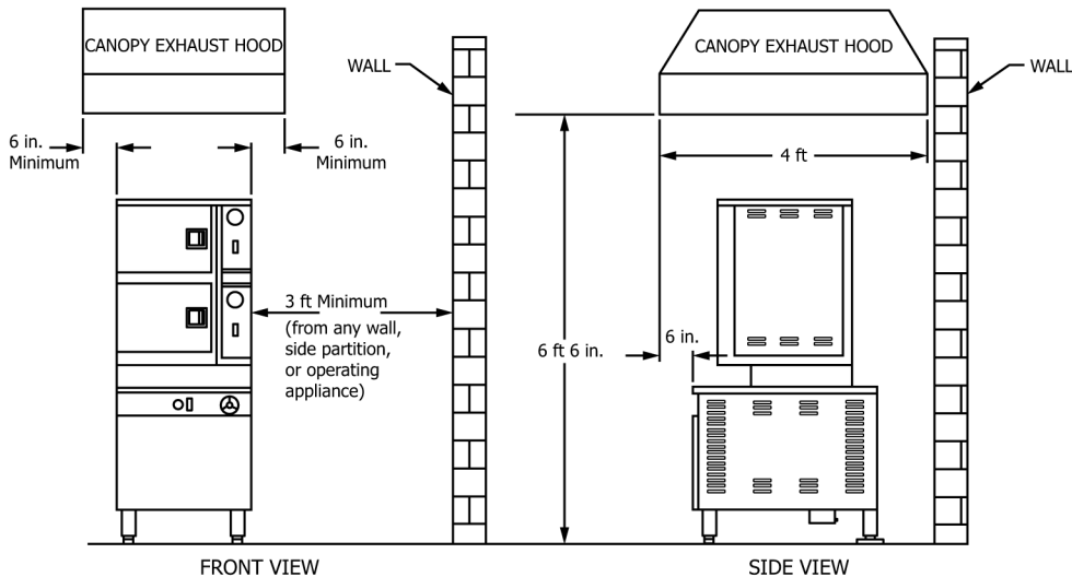
FIG. 3 Equipment Configuration
