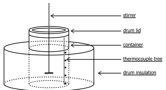
FIG. 1 Water-Bath Calorimeter
