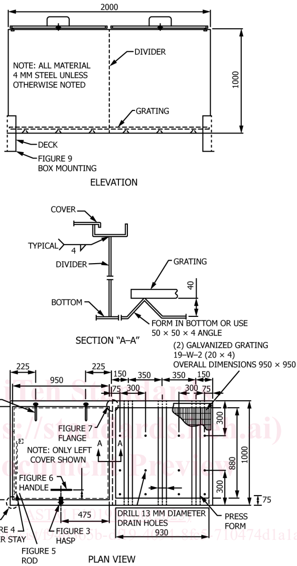
FIG. 1 Steel Deck Gear Stowage Box
