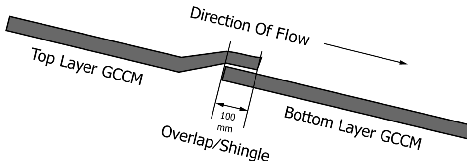
FIG. 32 Proper Shingled Joint of GCCM with Respect to Water Flow
