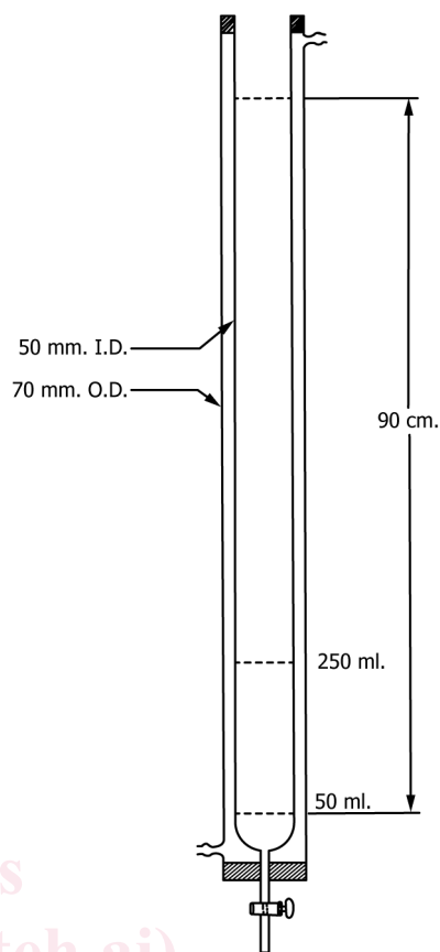
FIG. 2 Foam Receiver
