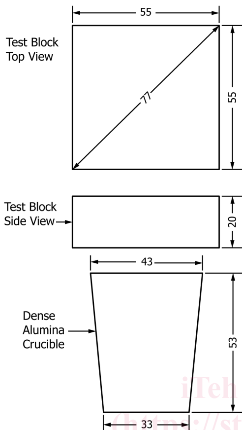
FIG. 1 Crucible-Cover Assembly
