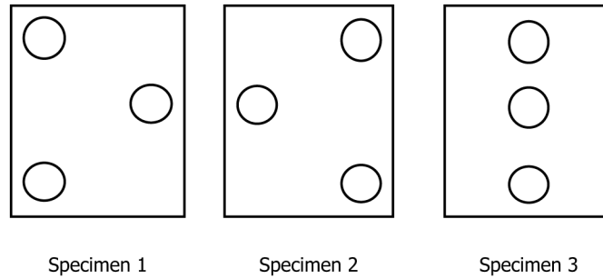
FIG. 2 Impact Locations for Small Missile Test (Each Type of Infill)
