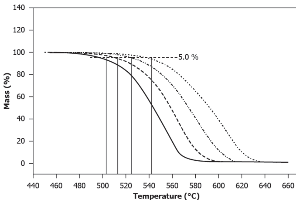
FIG. 1 Examples of Mass Loss Curves at the Following Heating Rates: 1^{\circ}\text{C}/\text{min} , 2^{\circ}\text{C}/\text{min} , 5^{\circ}\text{C}/\text{min} , 10^{\circ}\text{C}/\text{min} , 5.0\%
