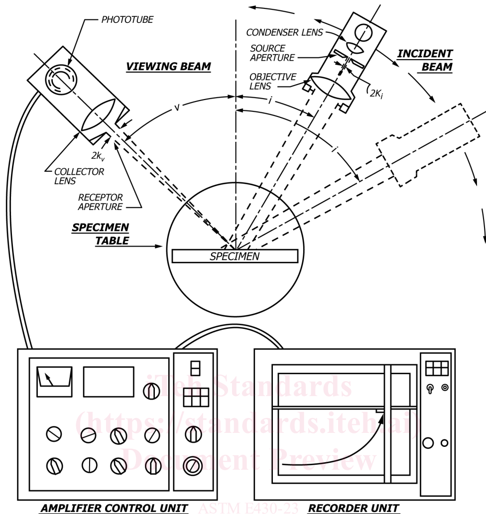
FIG. 5 Recording Goniophotometer Showing Viewing Angle, v , Incidence Angle, i , and Their Respective Field Angles, 2K_v and 2K_i
