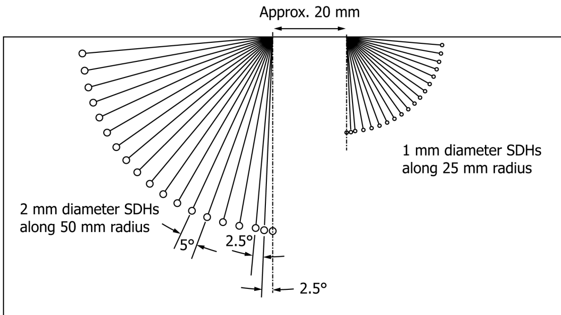
NOTE 1—Block dimensions 150 mm by 75 mm by 25 mm (typical) FIG. A2.1 Beam Steering Assessment Block—Constant Sound Path
