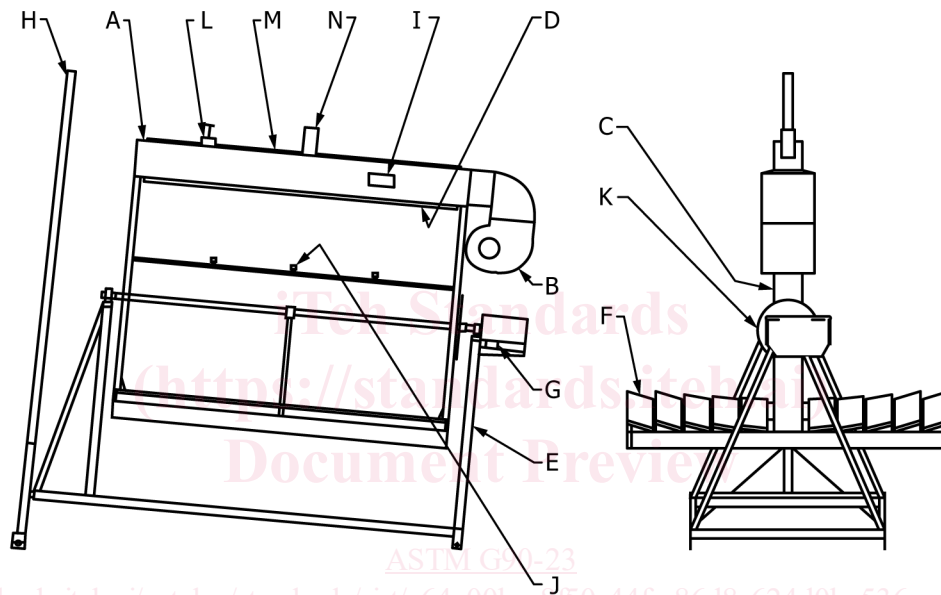
FIG. 1 Schematic of Fresnel-Reflecting-Linear Fresnel Reflector Concentrator Accelerated Weathering Machine Single Axis Tracking
