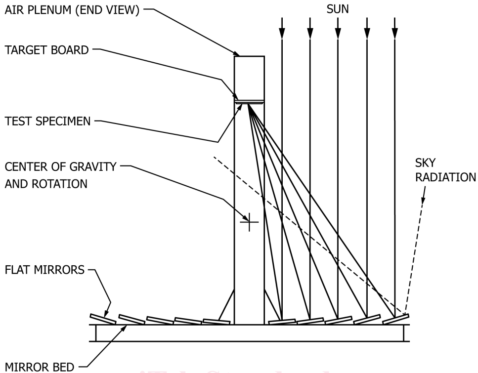
FIG. 3 Schematic of Optical System for a Linear Fresnel Reflecting Reflector Concentrator Accelerated Weathering Machine
