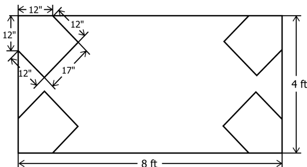
FIG. 2 Cutting Diagram
