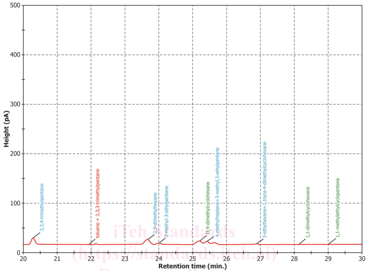
FIG. X1.3 Example Chromatogram Belonging to Report Data of Table X1.1 from 20 min to 30 min
