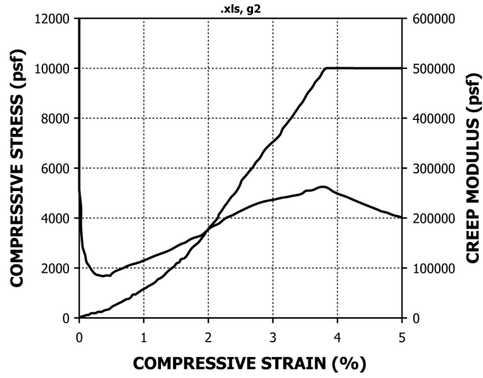
FIG. X1.2 Stress and Secant Modulus versus Compressive Strain
