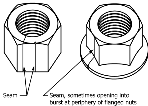
FIG. 6 Typical Seams in Nuts
