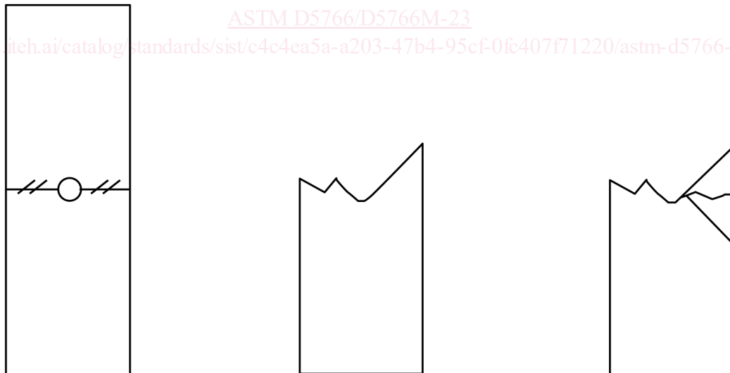
LGM Laminate tensile failure laterally across the center of the hole. Splits and delaminations may be present.
