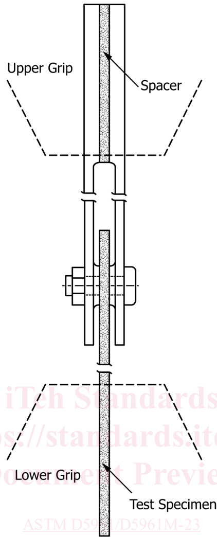
FIG. 43 Fixture Assembly for Procedure A
