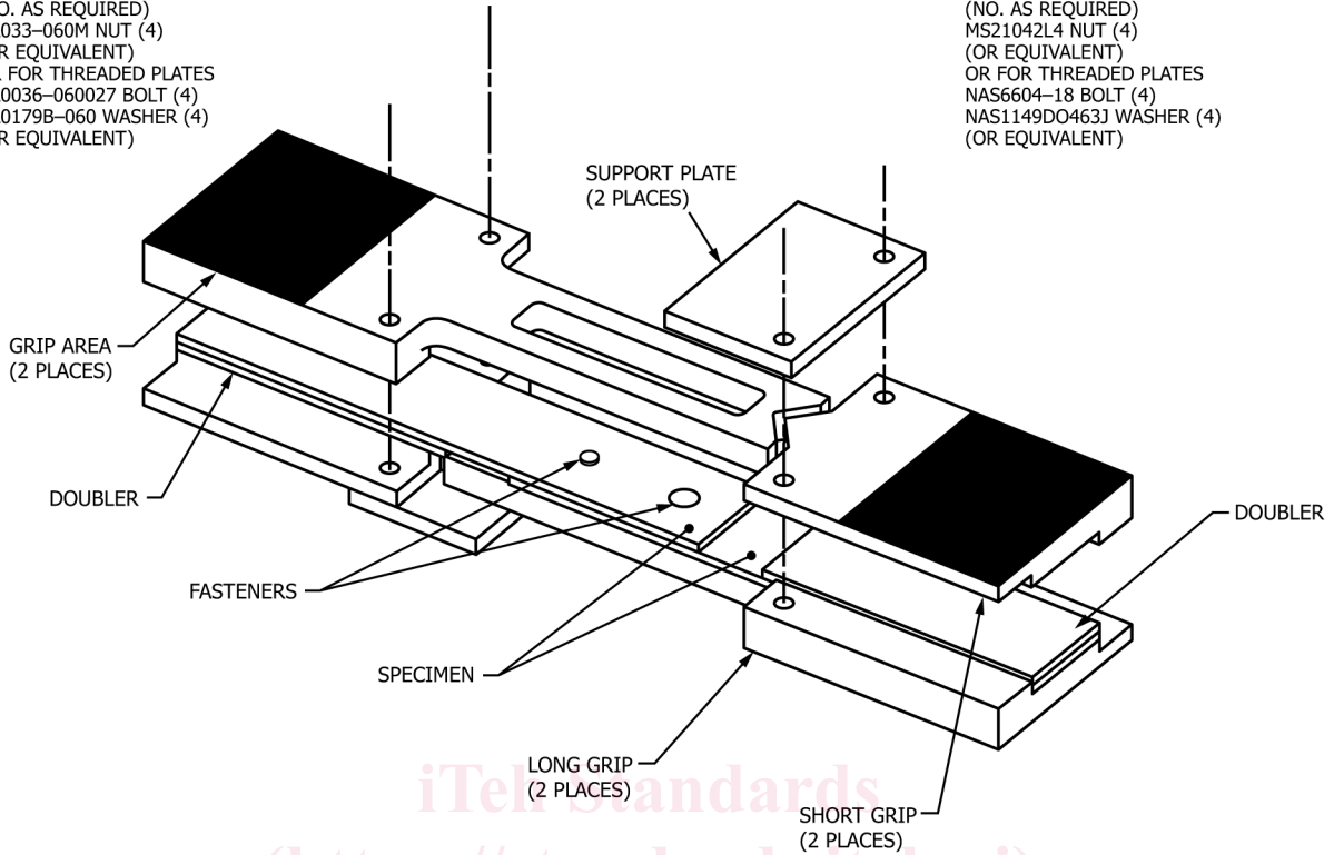
FIG. 98 Support Fixture Assembly for Procedure B
