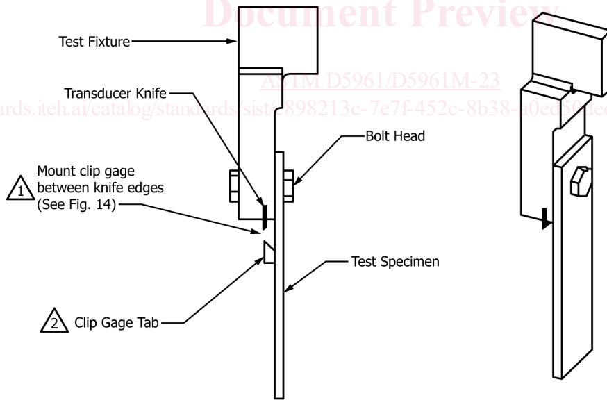
FIG. 98 Support Fixture Assembly for Procedure B
