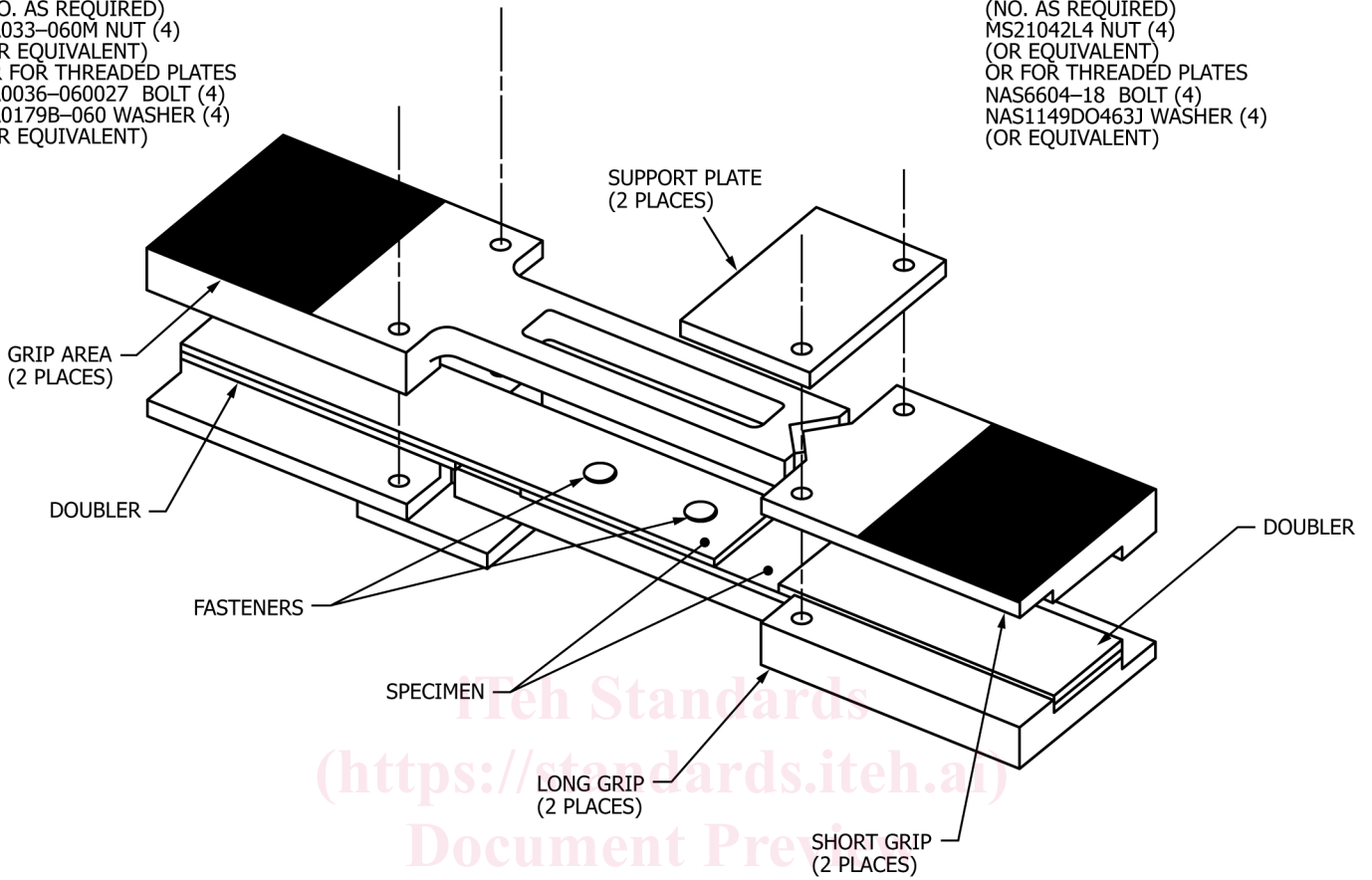
FIG. 87 Support Fixture Assembly for Procedure B (for details of the Support Fixture, see Test Method D5961/D5961M)
