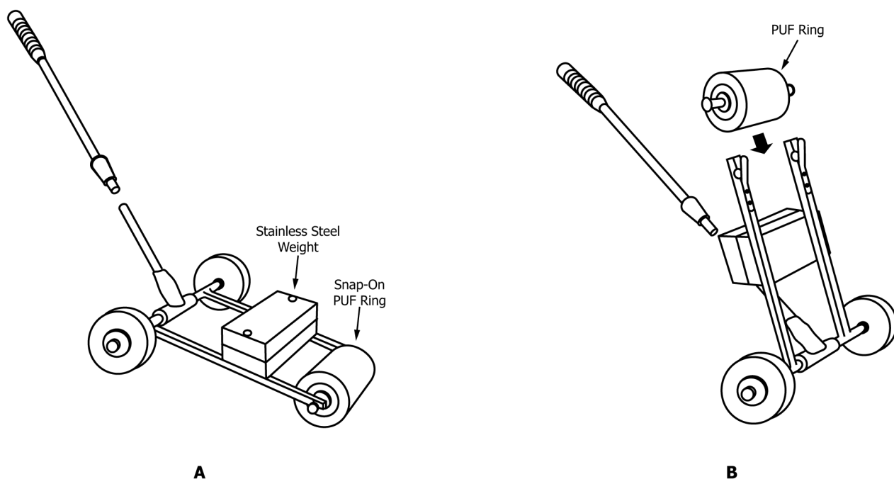
FIG. 1 PUF Roller: (A) In Position for Sampling; (B) Axle Cylinder/Frame Assembly
