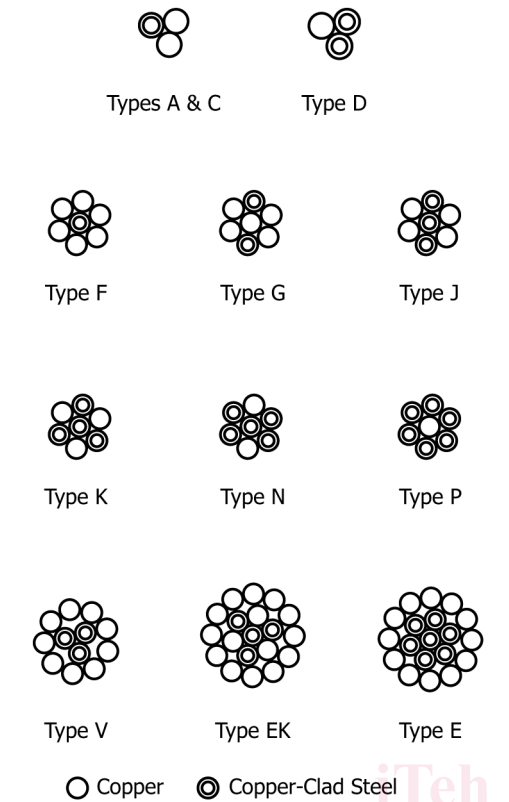
FIG. 1 Standard Types of Composite Conductors
