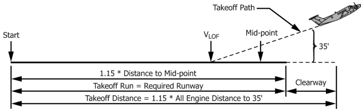
FIG. 4 Takeoff Run – All Engines Operating
