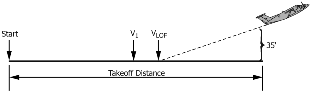
FIG. 1 Takeoff Distance with a Critical Loss of Thrust Recognized at V1
