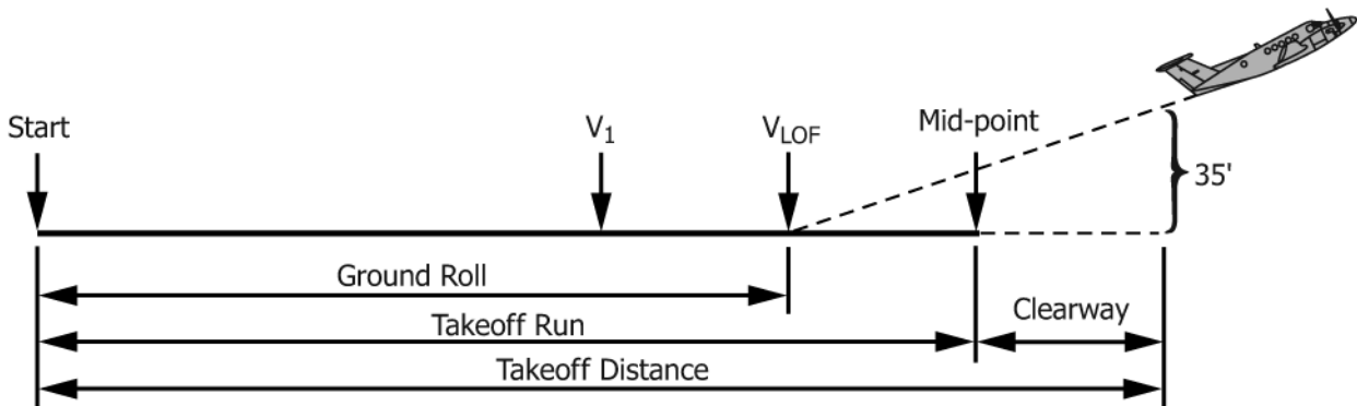
FIG. 3 Takeoff Run - Critical Loss of Thrust Recognized at V1
