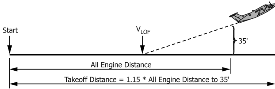
FIG. 2 Takeoff Distance - All Engines Operating
