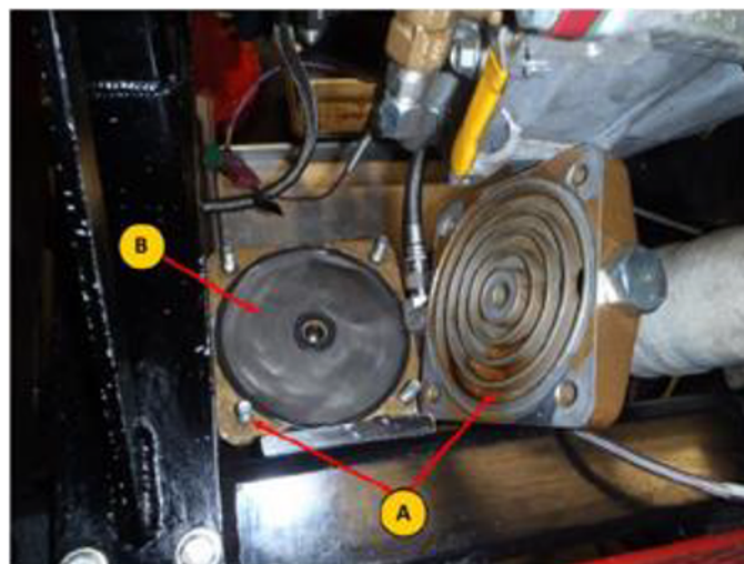
FIG. 4 Disassembled Oberg Filter Housing (A) with Filter Element (B)
