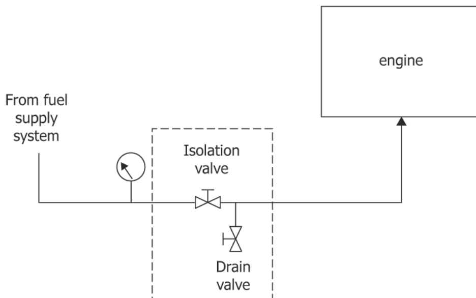
FIG. 1 Fuel System Isolation and Drain Valves
