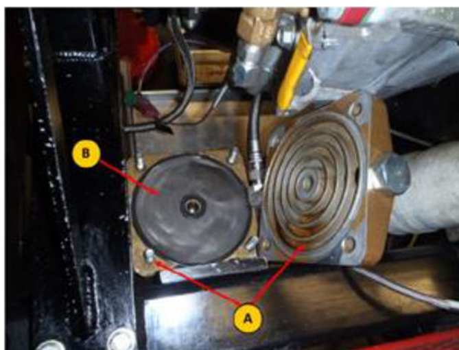
FIG. 4 Disassembled Oberg Filter Housing (A) with Filter Element (B)
