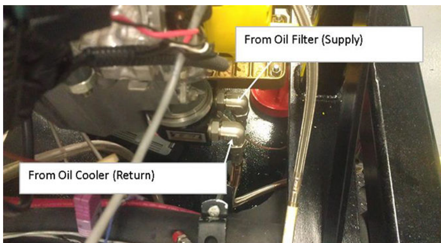
FIG. 3 Remote Oil Filter Housing Adapter
