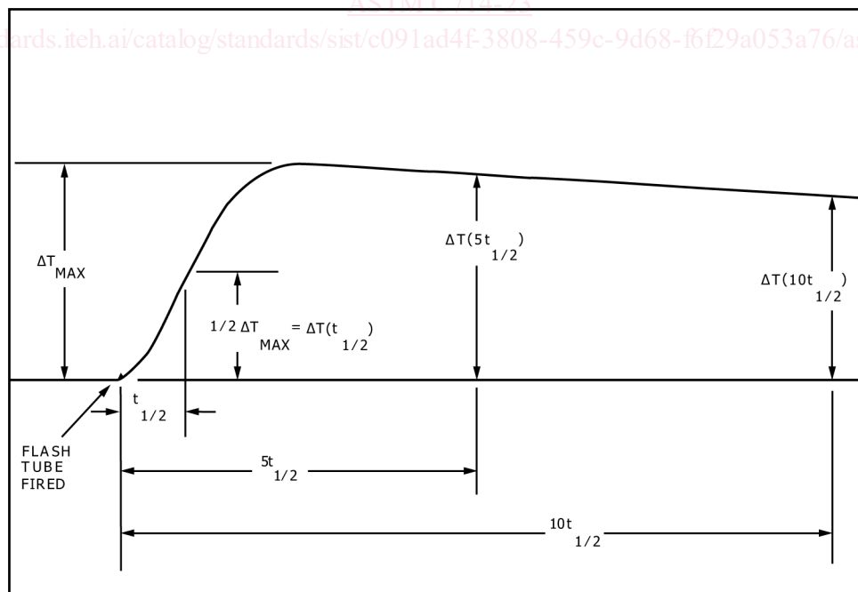
FIG. 2 Example of Oscilloscope Trace a Data Output Showing Parameters Used to Calculate Thermal Diffusivity
