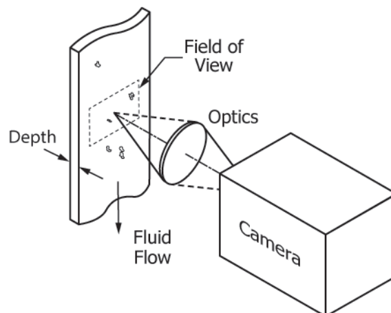
FIG. 2 Flow Cell
