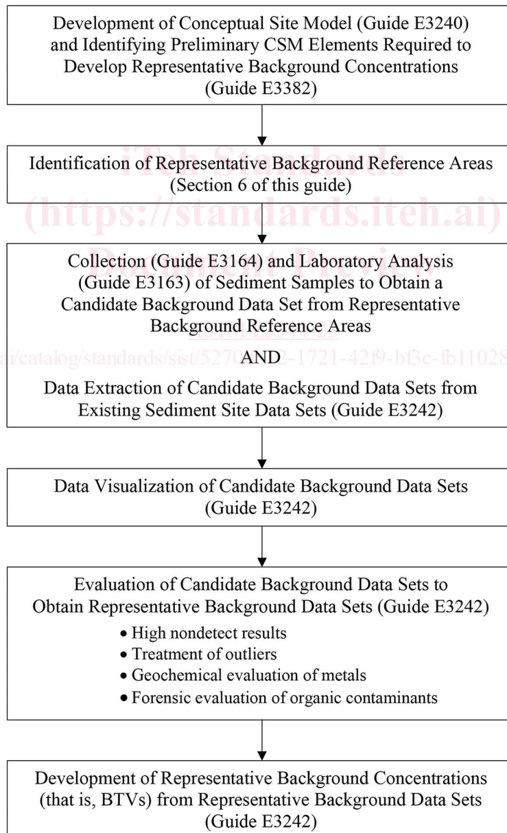
FIG. 1 Process to Determine/Develop Representative Sediment Background Concentrations (Modified from Guide E3242/E3382)
