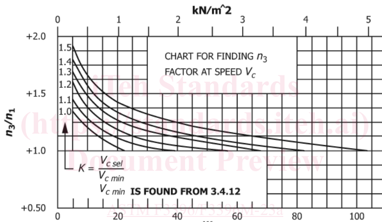
FIG. 2 Chart for Finding n_3 Factor at Speed V_C
