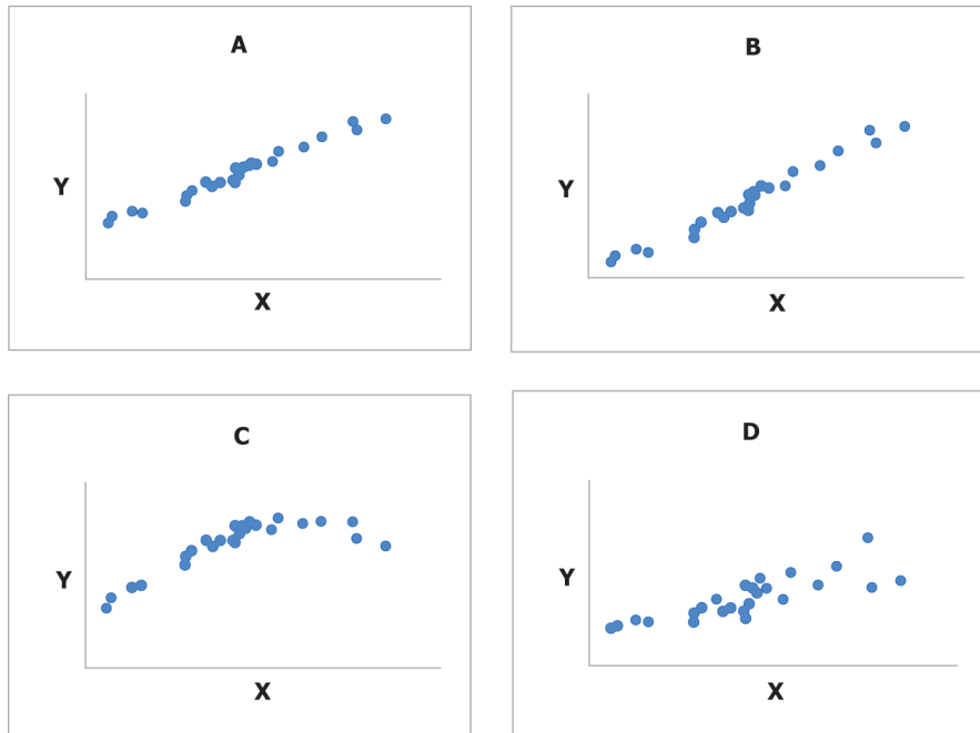
FIG. 1 Scatter Plots
