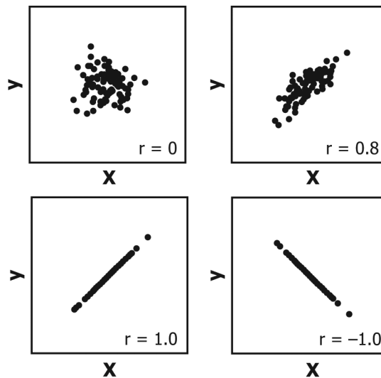
FIG. 5 Typical Scatter Plots for Selected Values of the Correlation Coefficient, r
