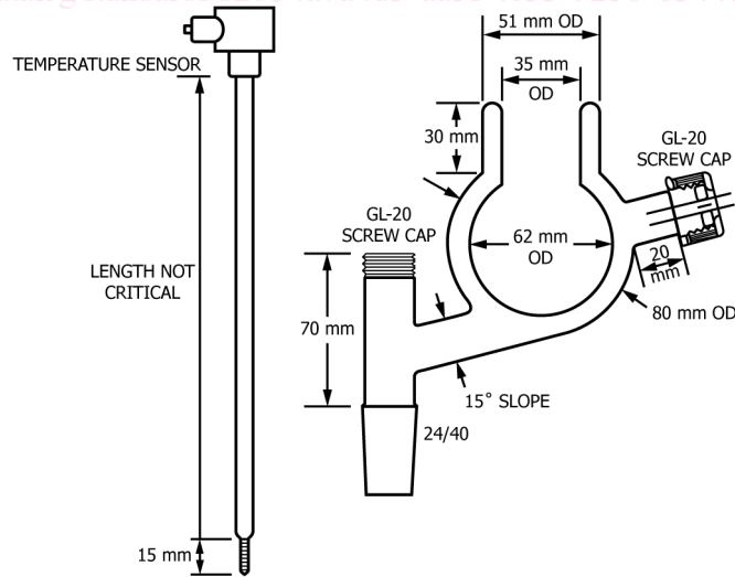
FIG. 4 Head Trap and Temperature Sensor
