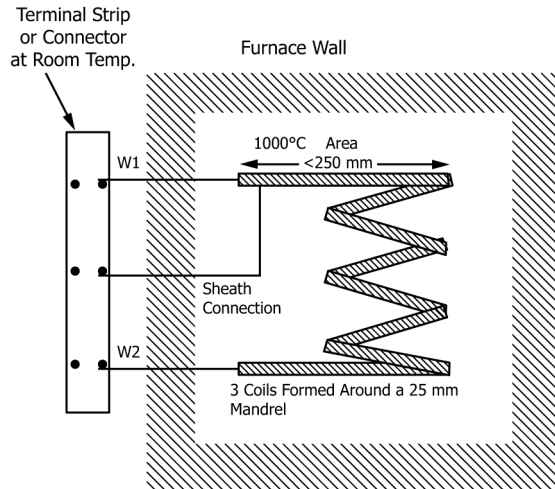
NOTE 1—The ends of the test specimen are not sealed, allowing water vapor to escape before measuring the insulation resistance FIG. 5 High Temperature Insulation Resistance Test, Insulation Contamination Other Than Moisture
