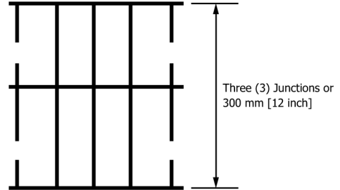
FIG. 3 Specimen Dimensions for Methods B and C
