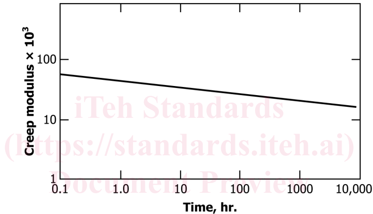
FIG. X2.4 Creep Modulus Versus Time on Logarithmic Coordinates
