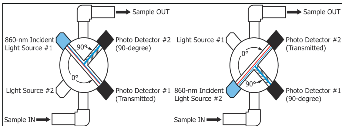
FIG. 3 Ratio Photoelectric Nephelometer (Multiple Beam Design)
